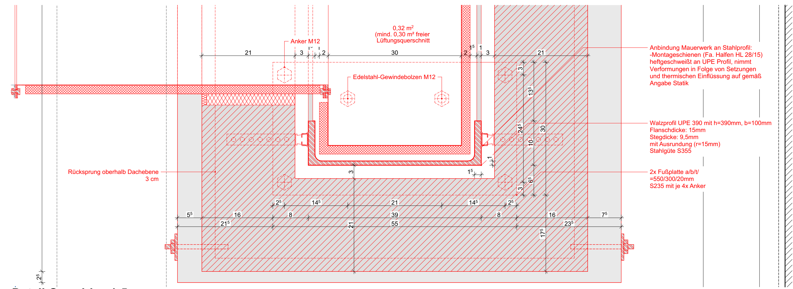
Detail Grundriss 1:5
